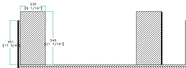
E-E VIEW
