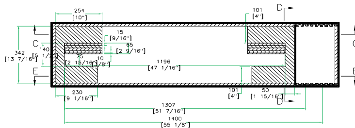
TOP VIEW OF BASE
