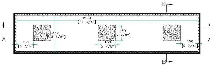
TOP VIEW OF COVER
