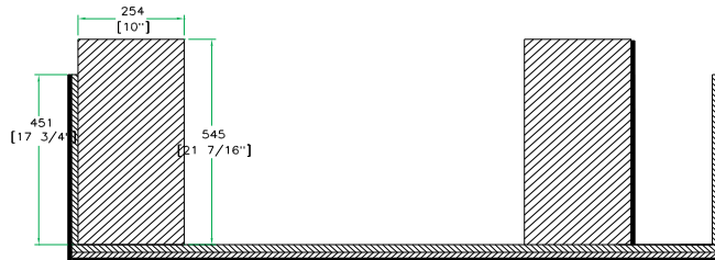
C-C VIEW
