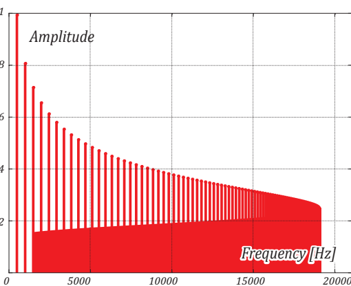
fig. 7: INHARMONIC SPECTRA RESULTING FROM POSITIVE (UPPER) AND NEGATIVE (LOWER) VALUES OF TENSION
