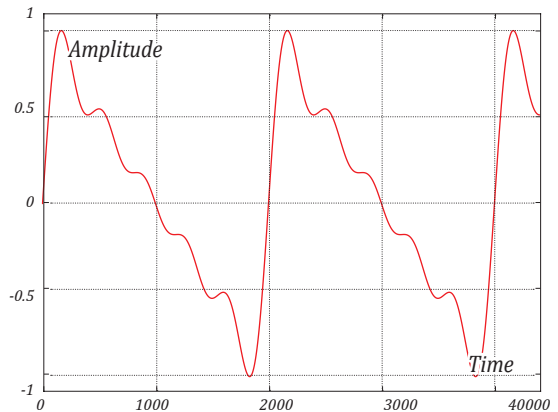
fig. 3b: SAWTOOTH WAVE AFTER LIMITING THE SPECTRUM TO THE INITIAL 5 PARTIALS
