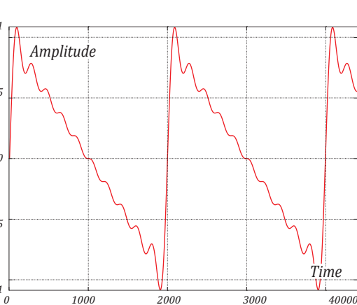
fig. 3a: SAWTOOTH WAVE AFTER LIMITING THE SPECTRUM TO THE INITIAL 10 PARTIALS
