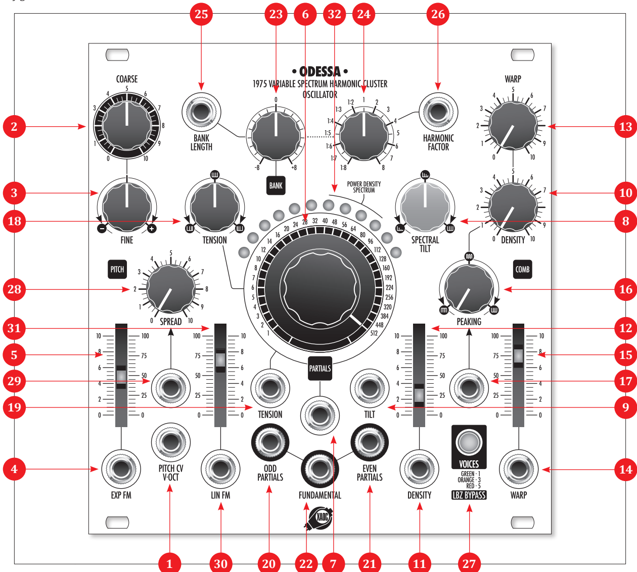
fig. 1: ODESSA FRONT PANEL LAYOUT AND CONTROLS
