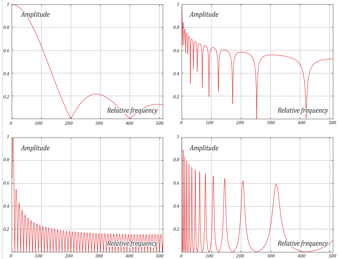
fig. 5: TILT + COMB FREQUENCY RESPONSE FOR LOW (UPPER) AND HIGH (LOWER) DENSITY VALUES
