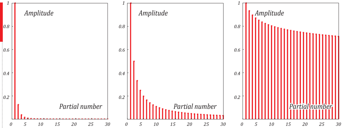
fig. 4: COMPARISON OF TILTED SPECTRA IN EXTREME AND MIDDLE POSITIONS OF THE TILT KNOB
