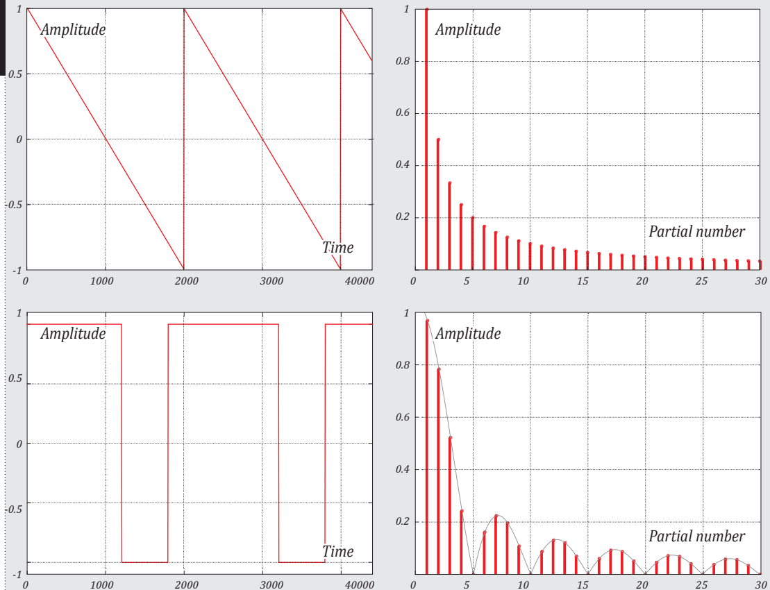
fig. 2: SAWTOOTH AND PULSE WAVEFORMS AND THEIR RESPECTIVE HARMONIC SPECTRA (TRUNCATED FOR CLARITY)
