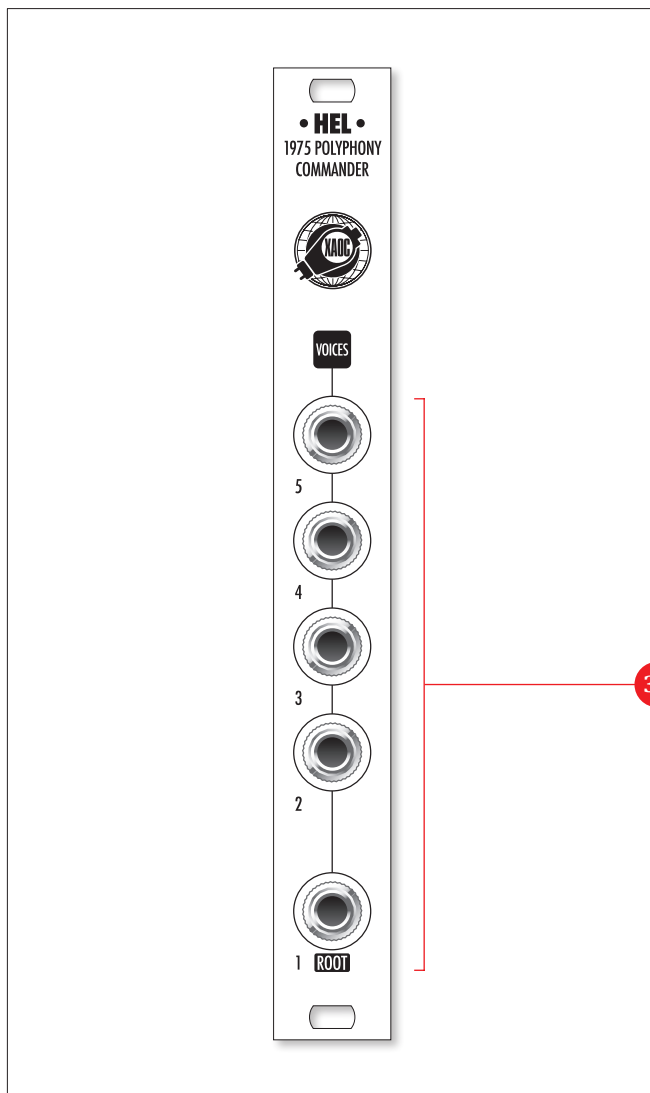
fig. 9: HEL FRONT PANEL LAYOUT AND CONTROLS
