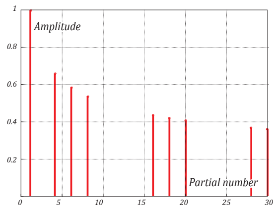
fig. 8: SIGNAL SPECTRA AT THE ODD PARTIALS AND EVEN PARTIALS OUTPUTS FOR LENGTH=3 AND FACTOR=2
