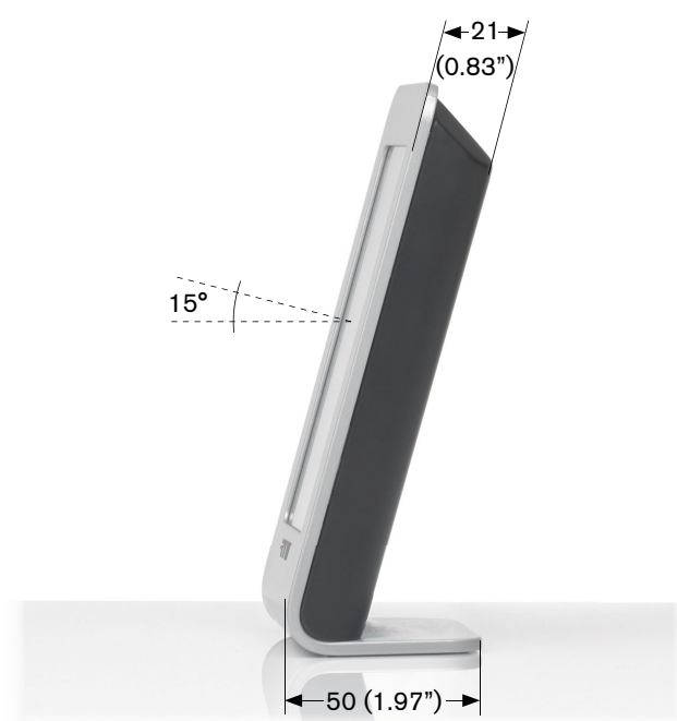
2 | Side view
